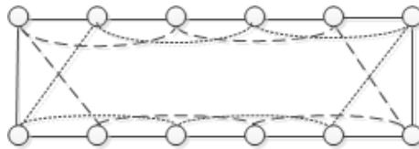
Figure 5: Dotted and dashed disjoint cycles of an even cycle.
