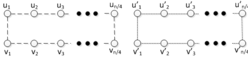
Figure 6: Vertices of dashed and dotted even cycles.
