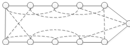
Figure 2: Solid and dashed cycles of C_{11} .
