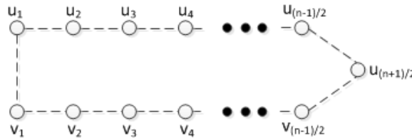
Figure 4: Vertices in the dashed cycle.
