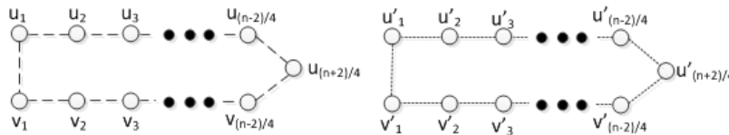
Figure 7: The dashed and dotted cycles when n \equiv 6 \pmod 8 .
